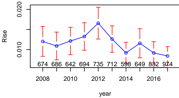
Pitch Type – SL – Mean Rise, by Year
