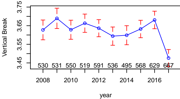
Mean Vertical Break, by Year
