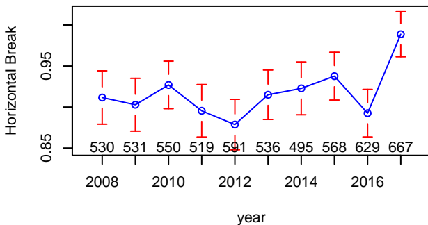
Mean Horizontal Break, by Year
