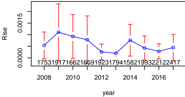
Pitch Type – FF – Mean Rise, by Year
