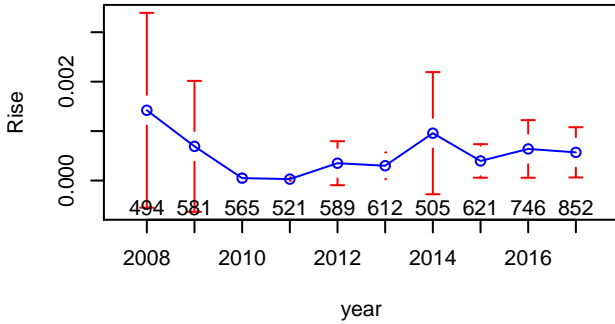
Pitch Type – FT – Mean Rise, by Year
