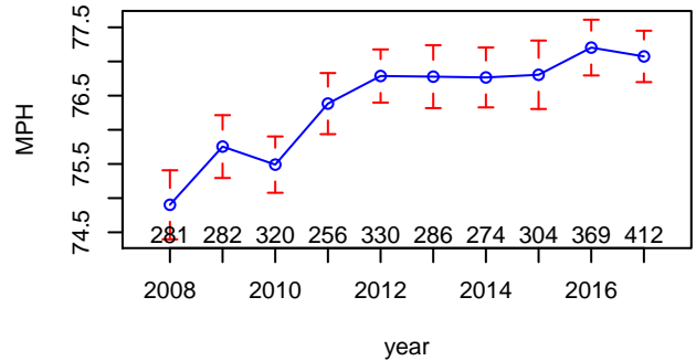
Mean Start Speed, by Year
