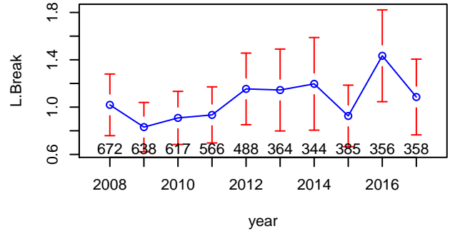
Mean Lateness of Break, by Year
