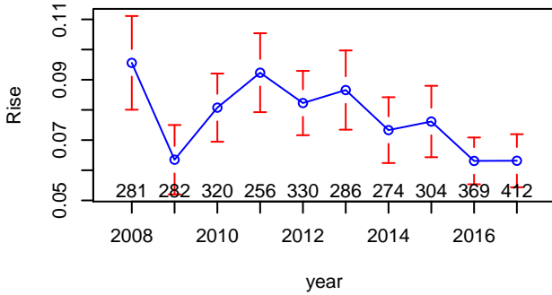
Pitch Type – CU – Mean Rise, by Year
