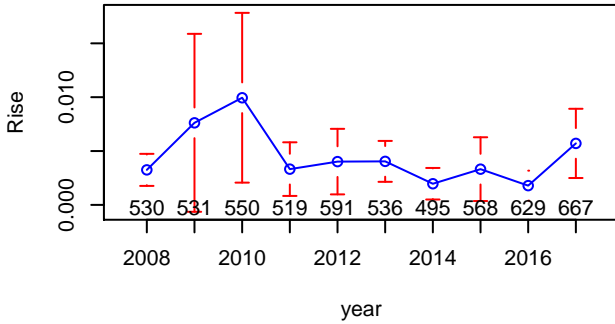
Pitch Type – CH – Mean Rise, by Year
