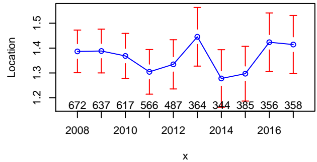
Mean Location, by Year
