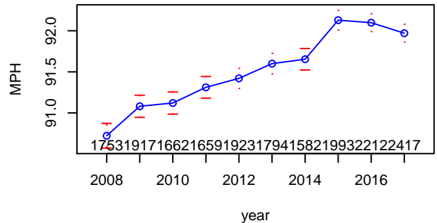
Mean Start Speed, by Year
