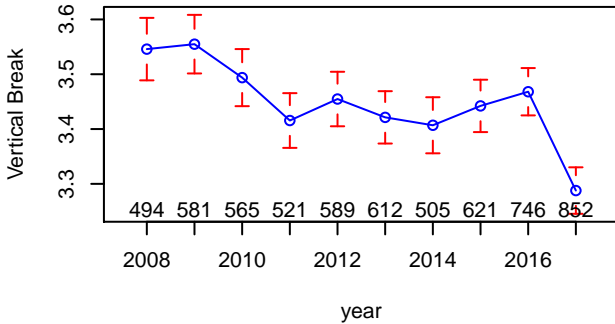
Mean Vertical Break, by Year
