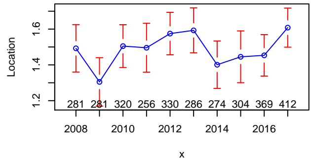
Mean Location, by Year
