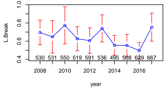
Mean Lateness of Break, by Year
