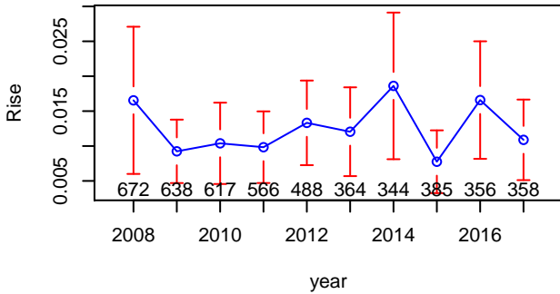
Pitch Type – SI – Mean Rise, by Year
